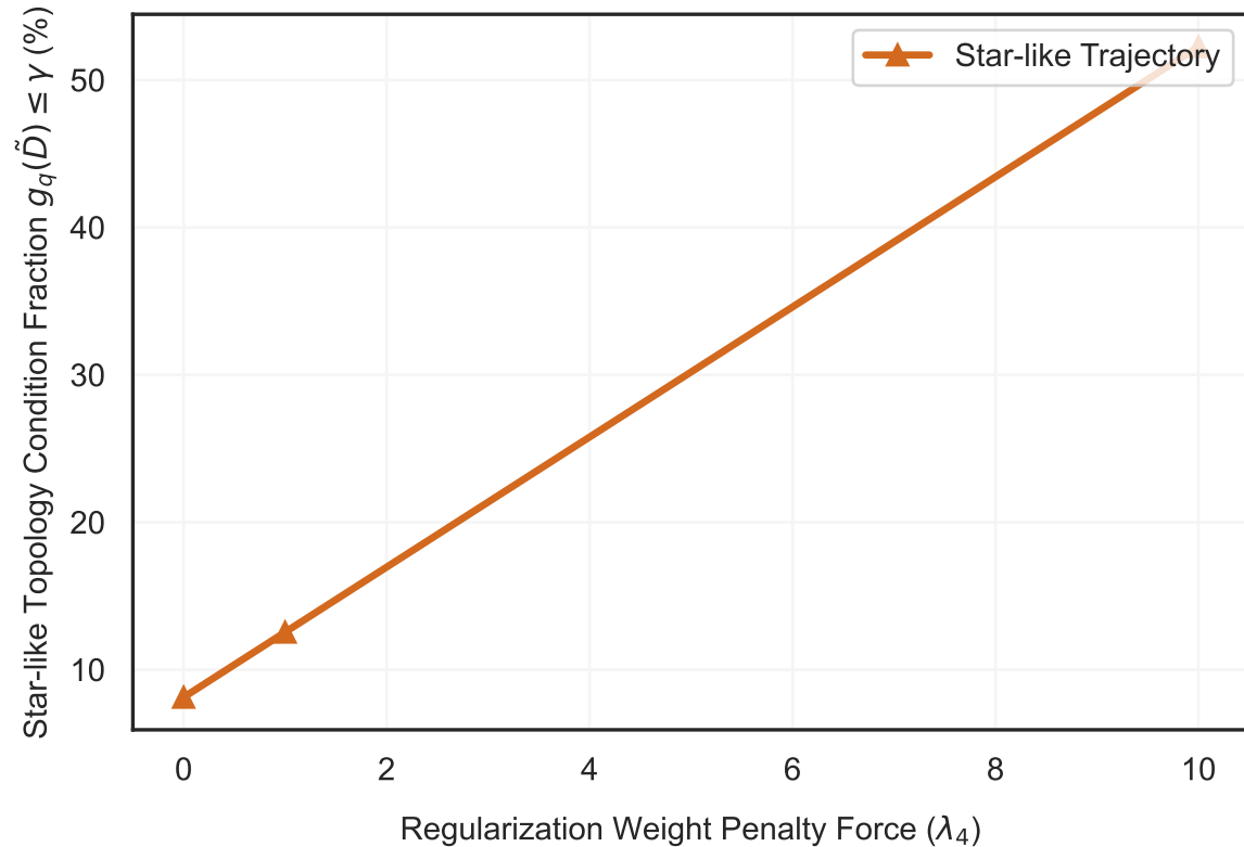
B. Latent Tree Topology Resolution Cliff
