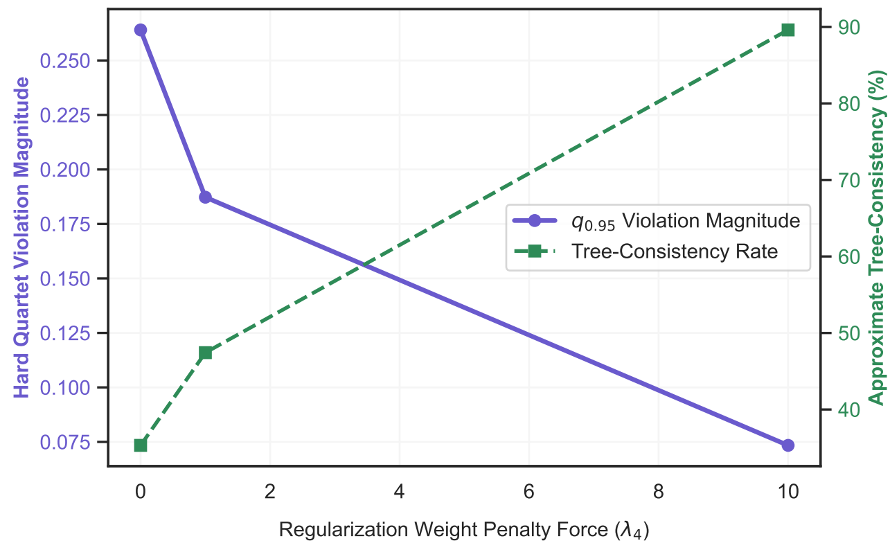
A. Structural Additivity Alignment
